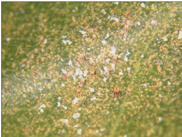
Oak spider mites and cast skins on upper leaf surface.
